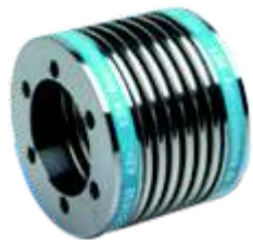
Coupling with flange mounting Torque range: 18 - 5000Nm
